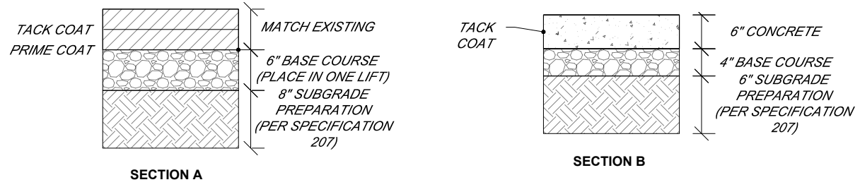
02 PAVEMENT & CONCRETE CROSS SECTIONS NOT TO SCALE
