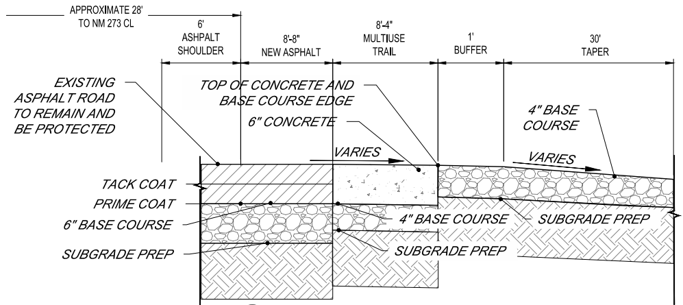
03 PAVEMENT & CONCRETE PROFILE NOT TO SCALE
